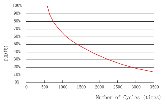
Cycle Service Life (25°C/77°F)
