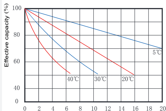
self discharge parameters characteristics
